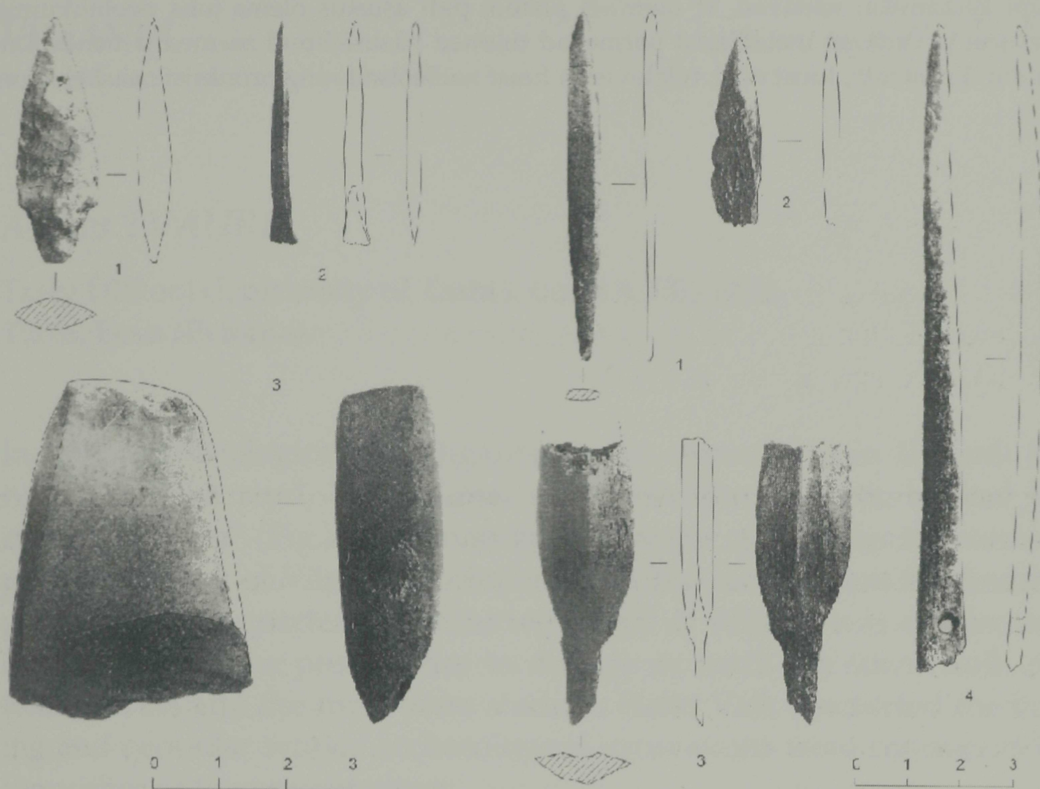
Fig. 2. Finds from the hill-fort of Narva Joaoru. (NLM.)
